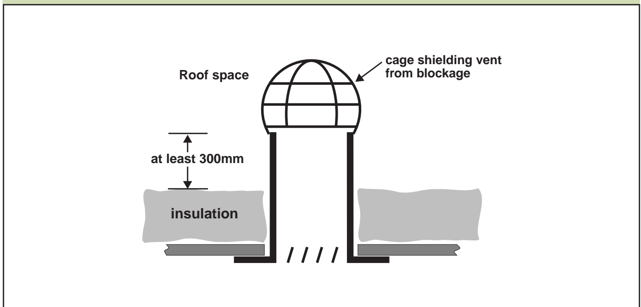
Diagram 1.5: Provision of ventilator communicating with a roof space (e.g. a loft)
